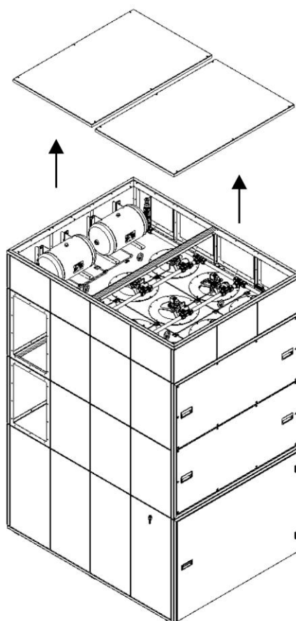
Fig. 17: Remover as chapas de cobertura
